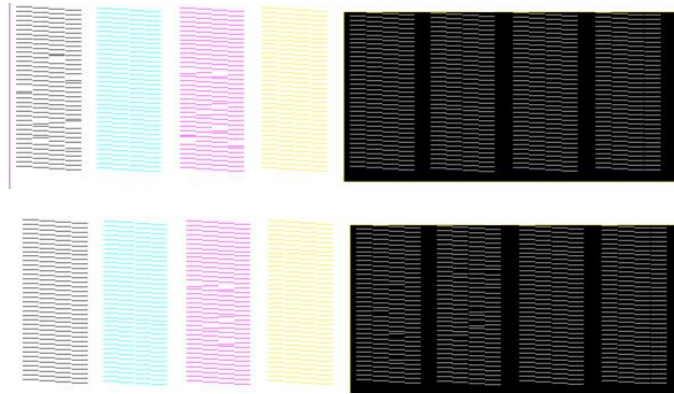
Abnormal Nozzle Check Pattern Fig.4 异常喷嘴 - 图 4 Oblique spray 喷嘴斜喷
